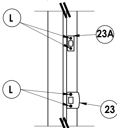
FRAME ANCHORING Masonry 2X buck construction
